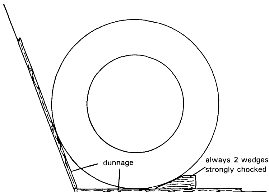
Figure 1 – Principle of dunnaging and wedging coils
