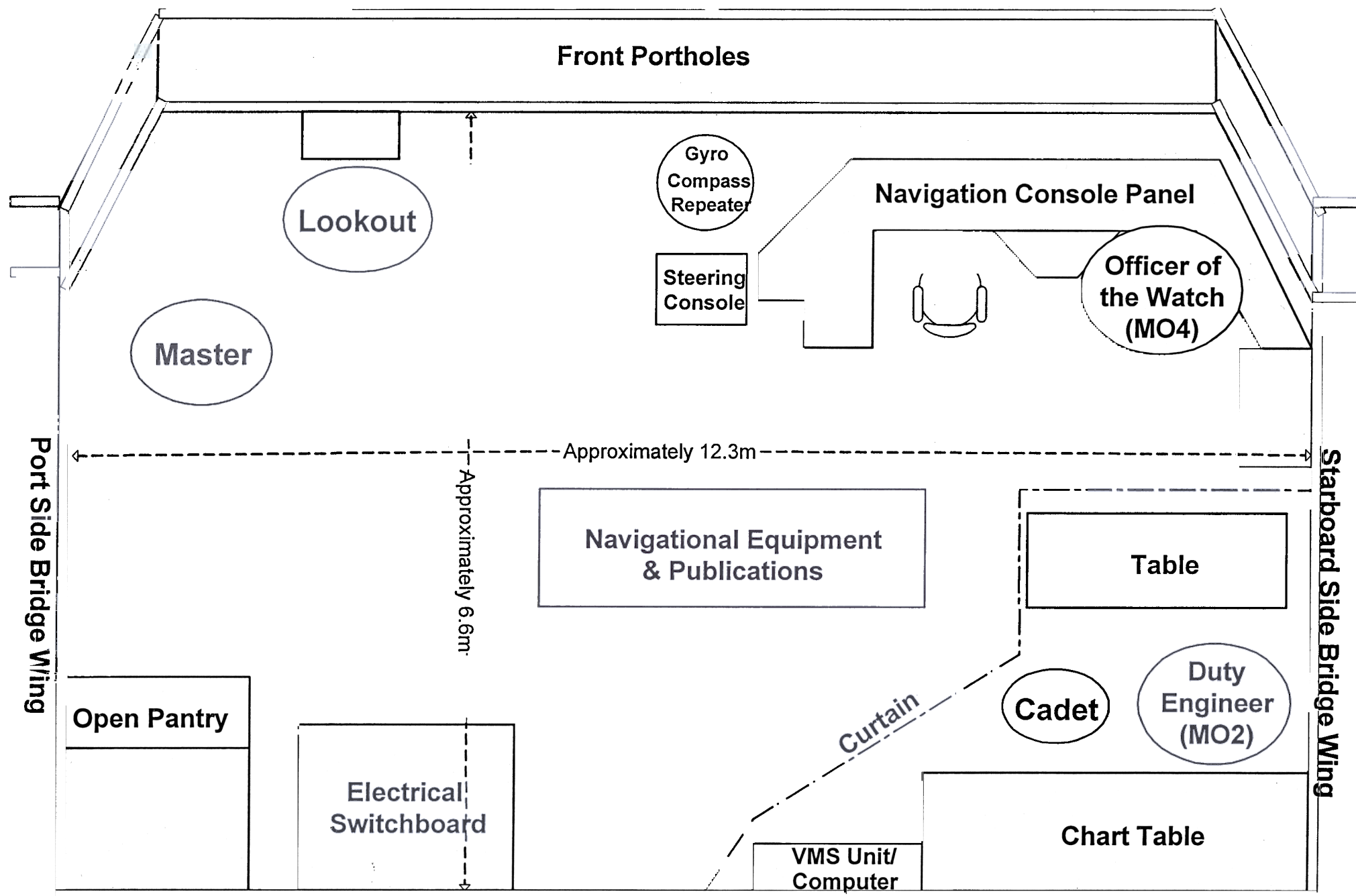
Schematic Layout of the Bridge of ANL Indonesia
