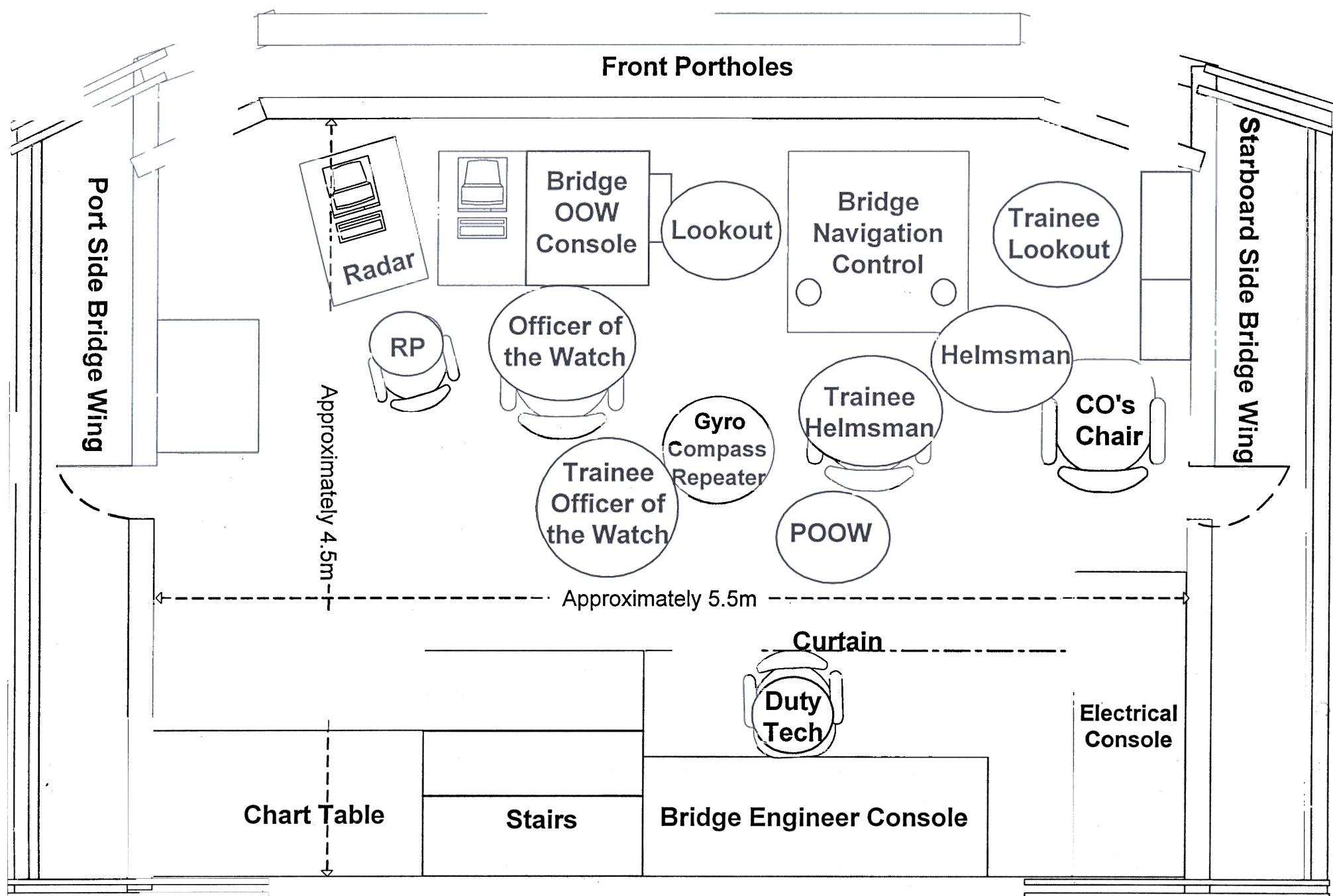
Schematic Layout of the Bridge of RSS Courageous
